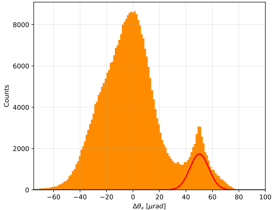
\Delta\theta_x distribution - (geometrically selected)
