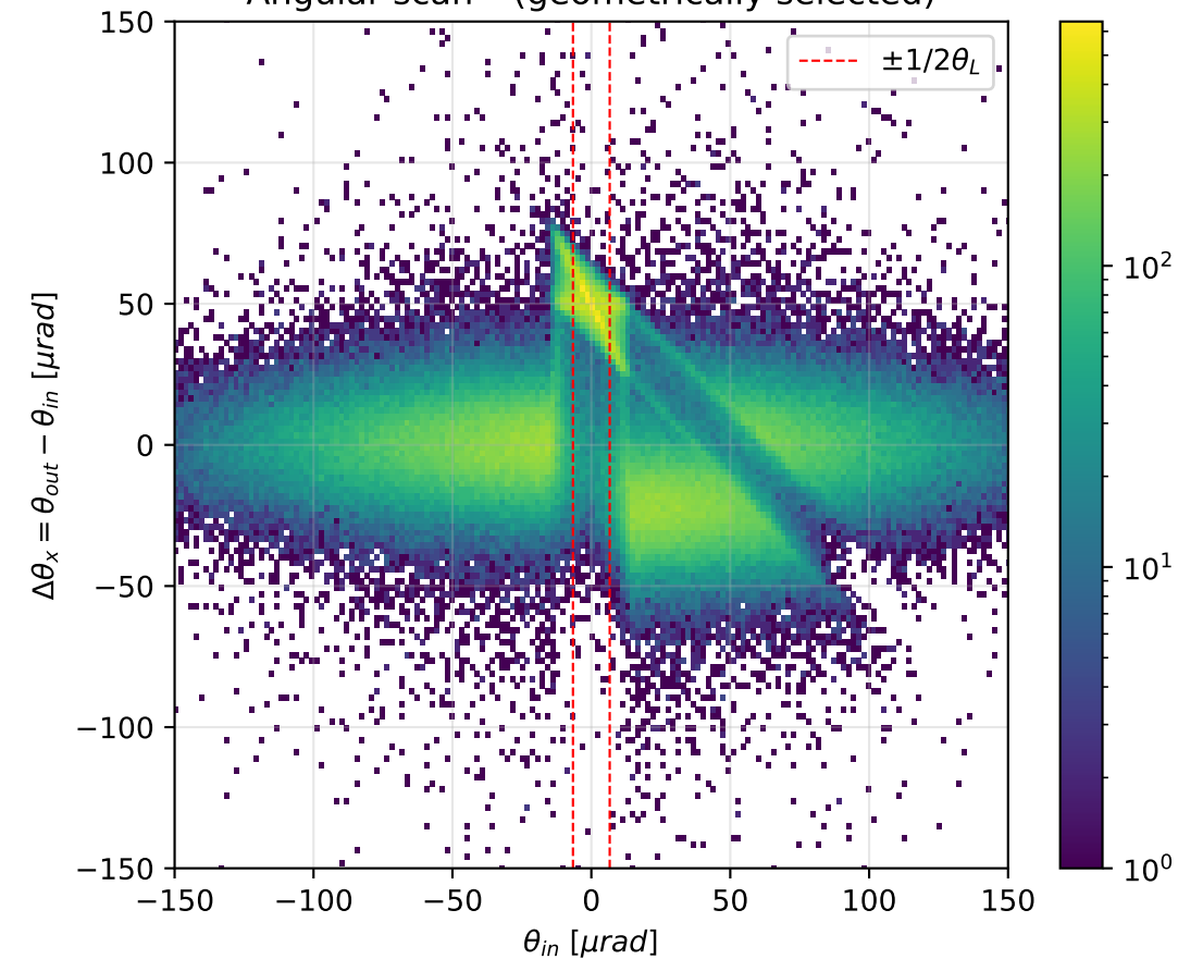
Angular scan - (geometrically selected)
